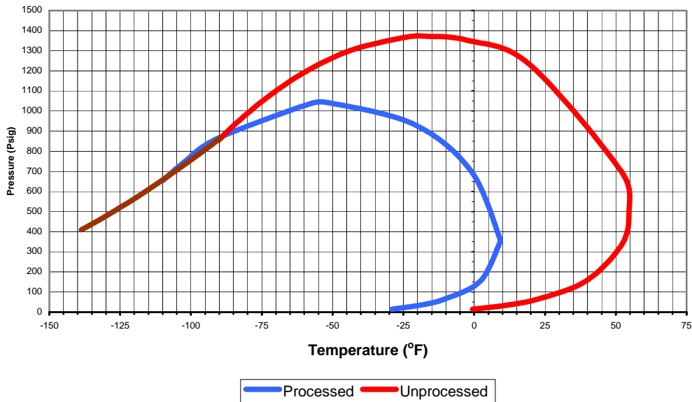
Figure 4-2 – Contrast of Unprocessed and Processed Natural Gas
